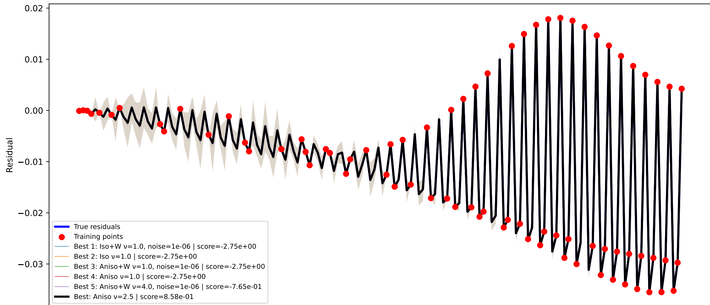
GPR kernel comparison node=18 RMSE=5.546e-06, train RMSE=1.060e-09
